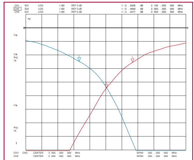
Crossover, 1 dB per Division
