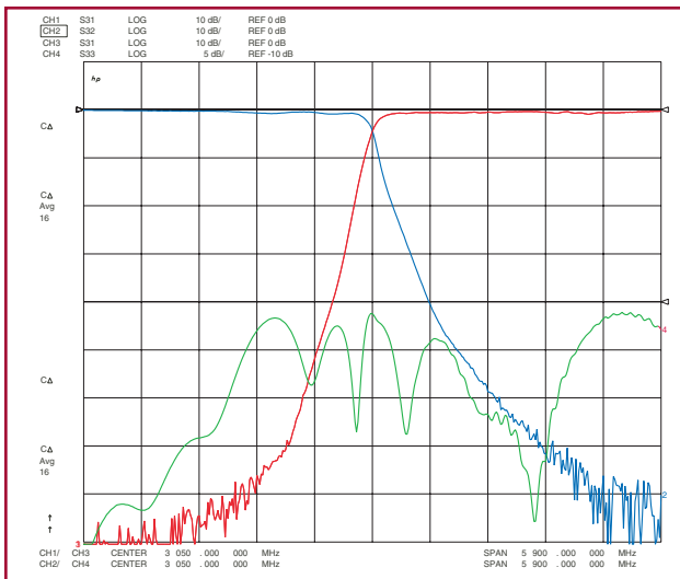
Crossover and VSWR 10 dB per Division
