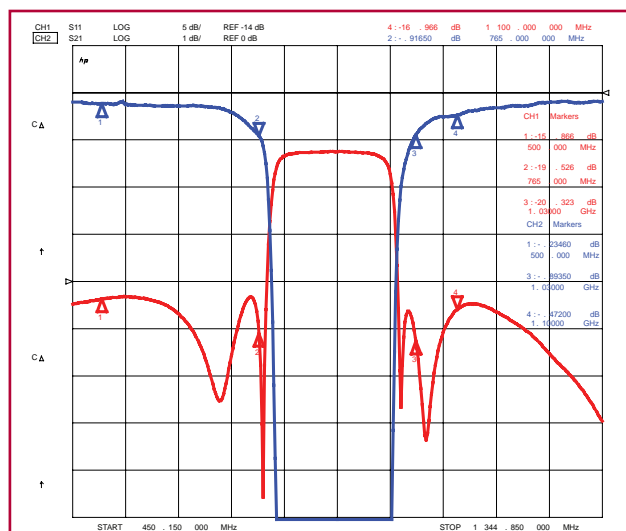
Insertion Loss/Return Loss
