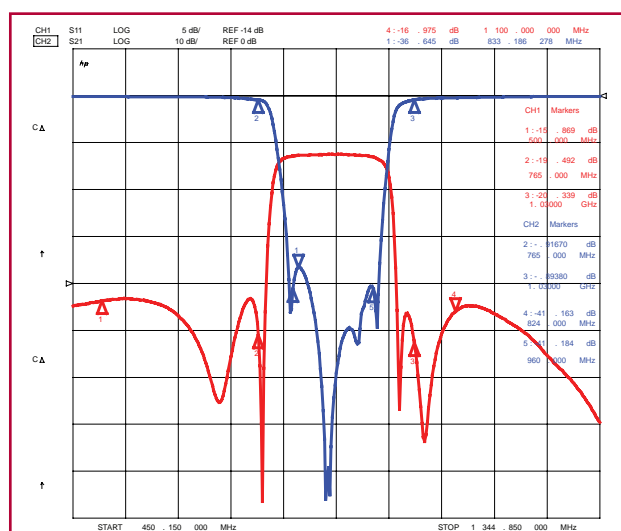
Rejection /Return Loss
